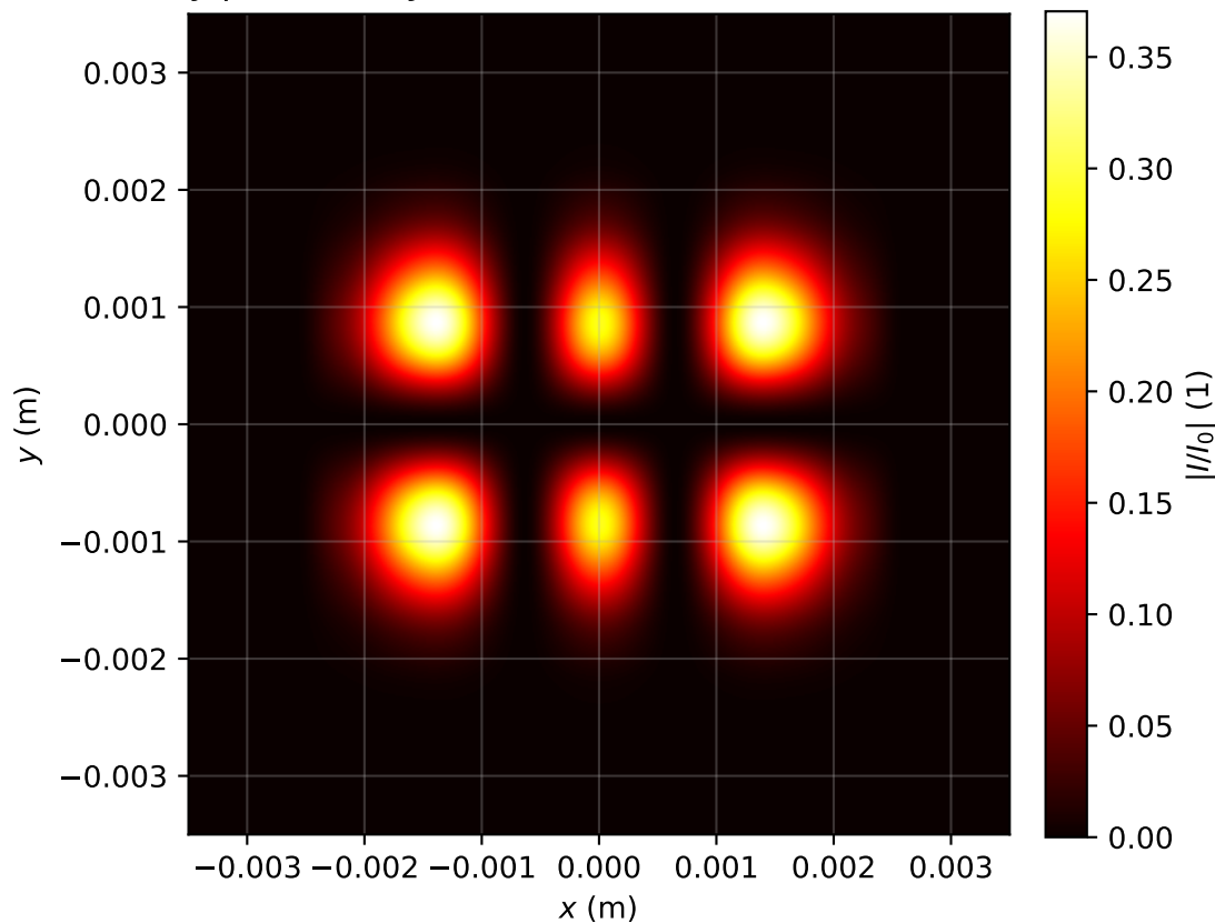
Intensity profile I(x, y, z = 2.946)/I_0 , P_{in}=1.0P_{cr} , artificial time
